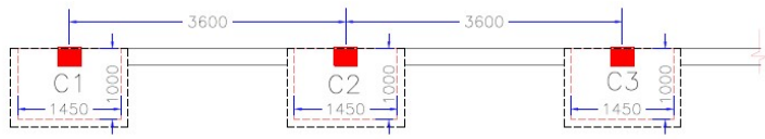
PLAN (LAYOUT OF COLUMNS & FOOTINGS @ GROUND FLOOR LVL.)
